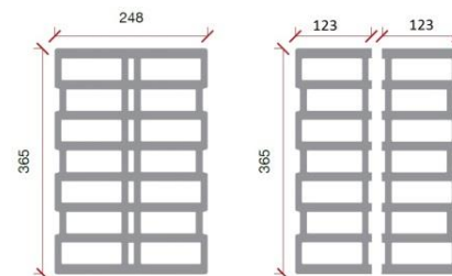
Porotherm 36,5 1/2 TermoPlus
